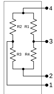
Equivalent Circuit
